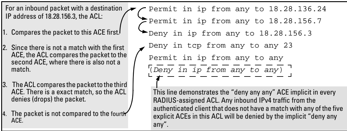
Figure 9-2. Example of Sequential Comparison
